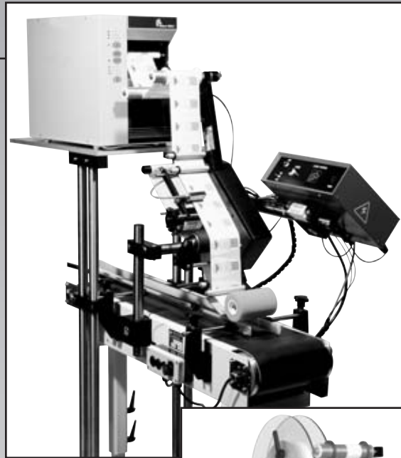
Mini System with LS75 and Loose Loop Option
